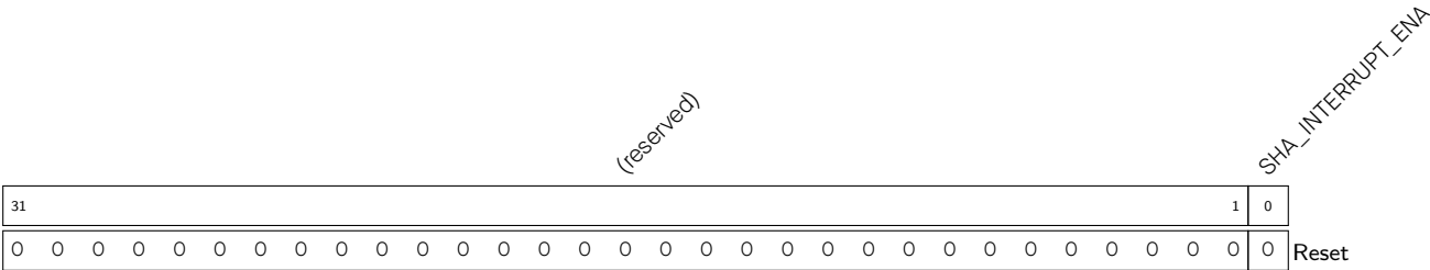
Register 21.7. SHA_INT_ENA_REG (0x0028)
