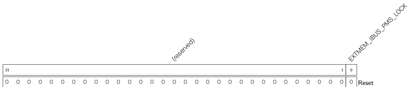
Register 14.79. EXTMEM_IBUS_PMS_TBL_LOCK_REG (0x00D8)
