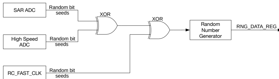
Figure 24.3-1. Noise Source
