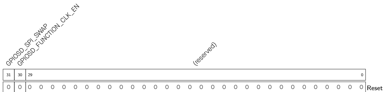
Register 5.25. GPIOSD_SIGMADELTA_MISC_REG (0x0024)
