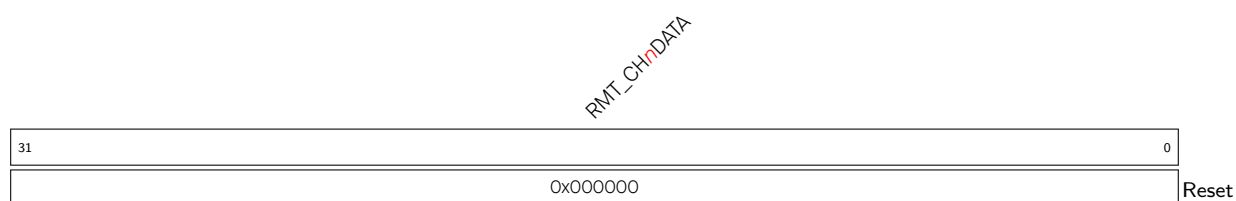
Register 33.1. RMT_CH n DATA_REG ( n = 0, 1 ) (0x0000, 0x0004)
