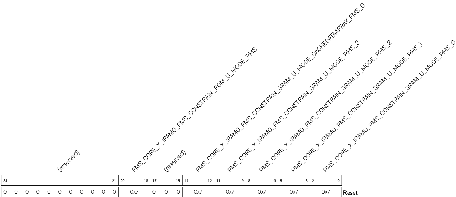
Register 14.29. PMS_CORE_X_IRAMO_PMS_CONSTRAIN_1_REG (0x00AC)
