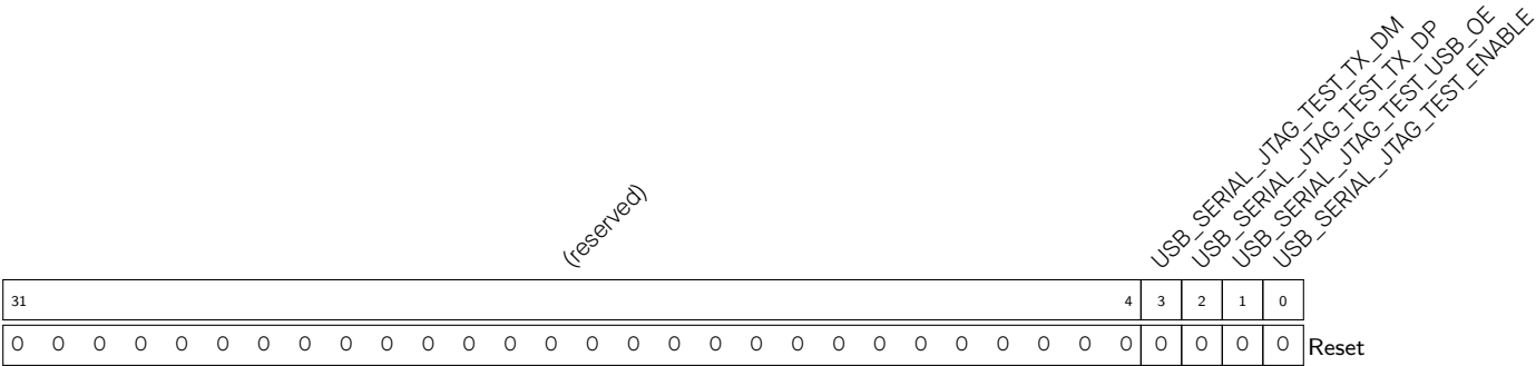
Register 30.3. USB_SERIAL_JTAG_TEST_REG (0x001C)
