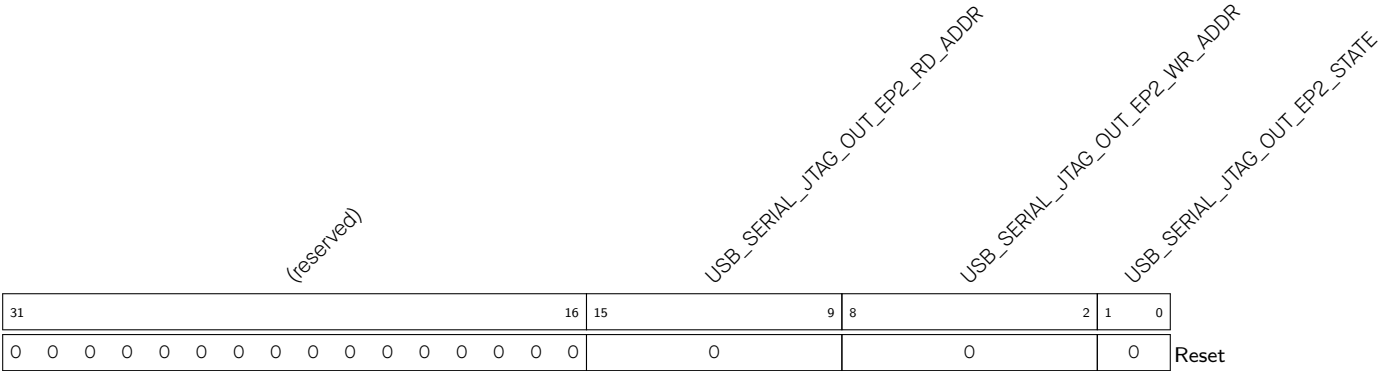
Register 30.15. USB_SERIAL_JTAG_OUT_EP2_ST_REG (0x0040)
