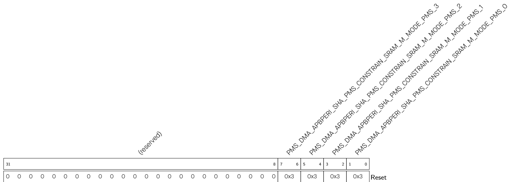
Register 14.17. PMS_DMA_APBPERI_SHA_PMS_CONSTRAIN_1_REG (0x0074)
