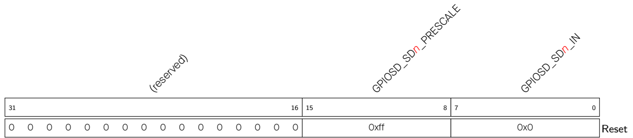
Register 5.23. GPIOSD_SIGMADELTA n _REG ( n : 0-3) (0x0000+4* n )
