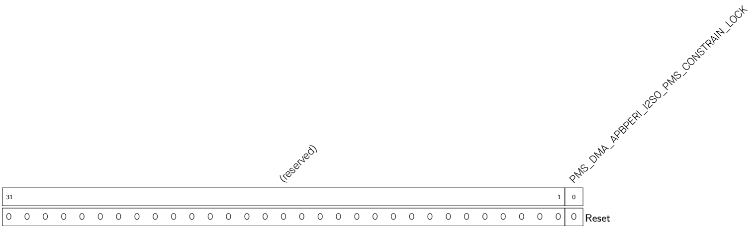
Register 14.12. PMS_DMA_APBPERI_I2SO_PMS_CONSTRAIN_O_REG (0x0048)
