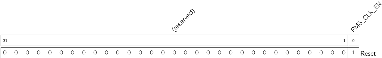
Register 14.71. PMS_CLOCK_GATE_REG_REG (0x0170)
