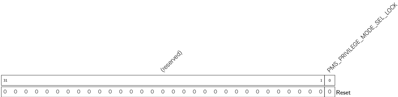
Register 14.1. PMS_PRIVILEGE_MODE_SEL_LOCK_REG (0x0008)
