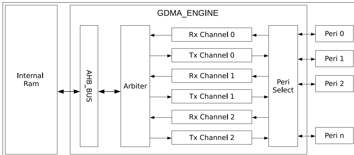
Figure 2.3-1. GDMA Engine Architecture
