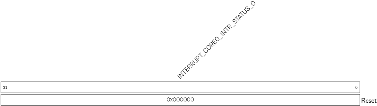
Register 8.52. INTERRUPT_CORE0_INTR_STATUS_O_REG (0x00F8)
