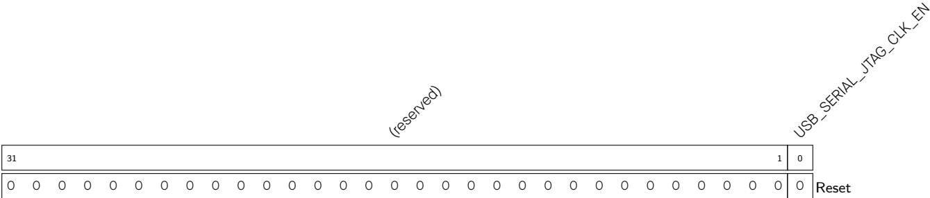
Register 30.4. USB_SERIAL_JTAG_MISC_CONF_REG (0x0044)
