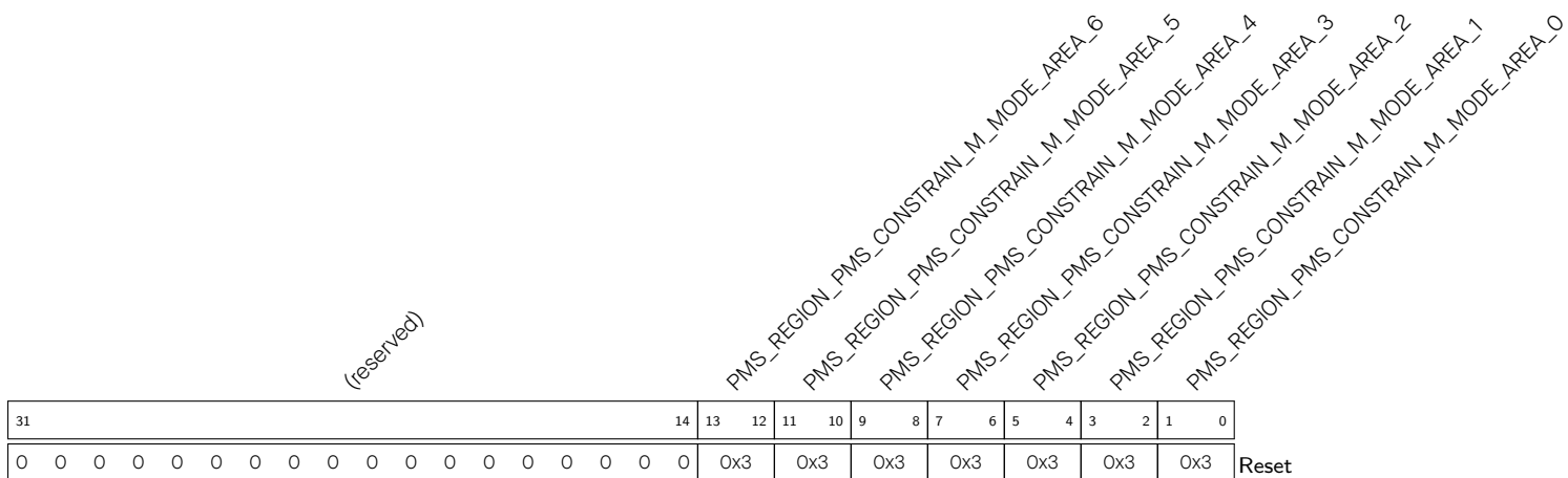
Register 14.49. PMS_REGION_PMS_CONSTRAIN_1_REG (0x0108)
