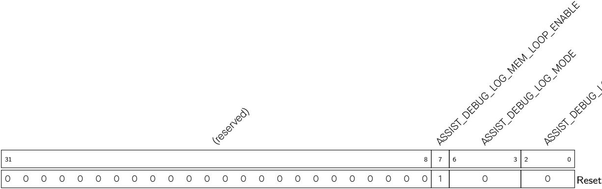
Register 17.21. ASSIST_DEBUG_LOG_SETTING_REG (0x0070)
