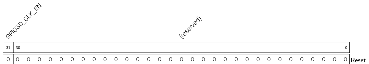
Register 5.24. GPIOSD_SIGMADELTA_CG_REG (0x0020)
