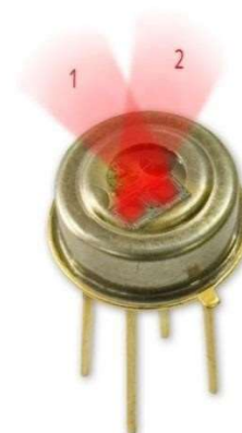
Figure 29 – Typical FOV of MLX90614xBA, Zone 1 & 2 identification relative to the alignment tab
