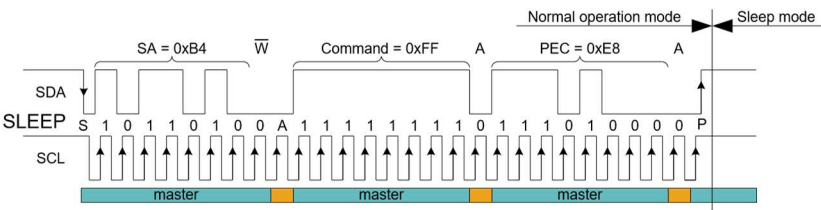
Figure 8 – Go to sleep mode command format (default SA = 0x5A, command = 0xFF, PEC = 0xE8)
