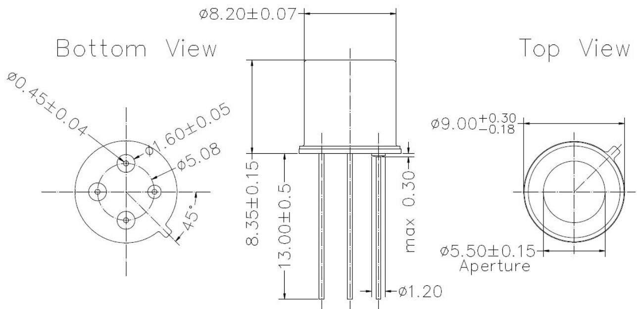
Figure 44 – Mechanical drawing of MLX90614xCH
